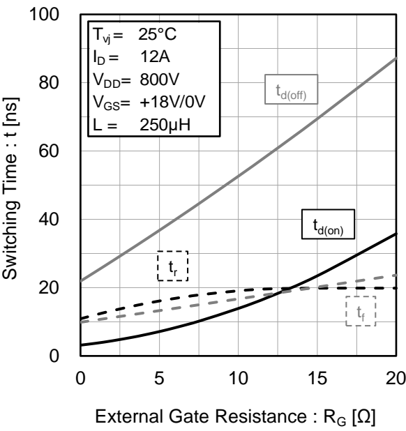
Fig.22 Typical Switching Time vs. External Gate Resistance
